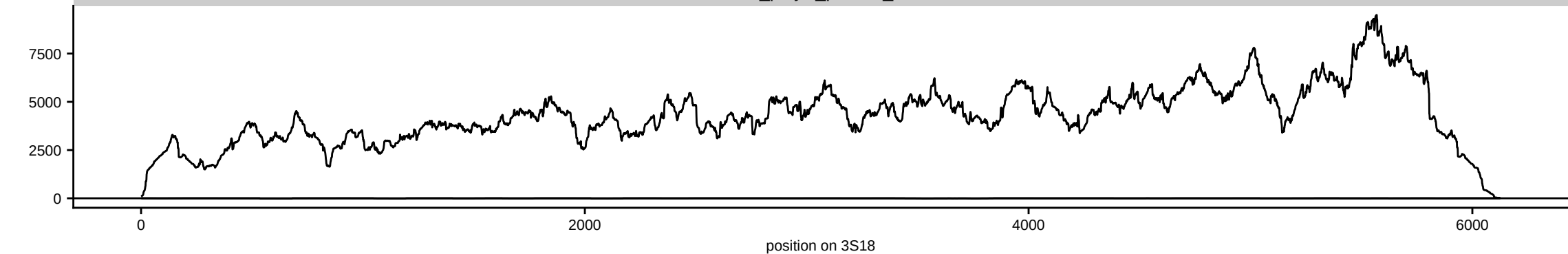
Ov_polyA_piwiKD_A
