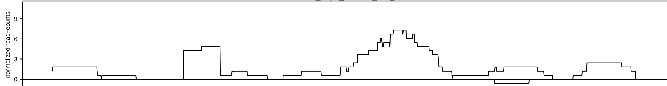
Ov_polyA_piwiKD_A
