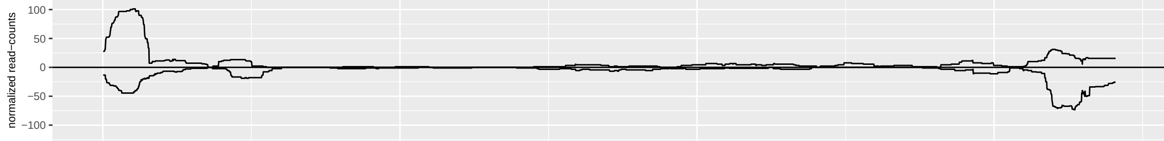
HsBam_polyA_moonKD_00h_A
