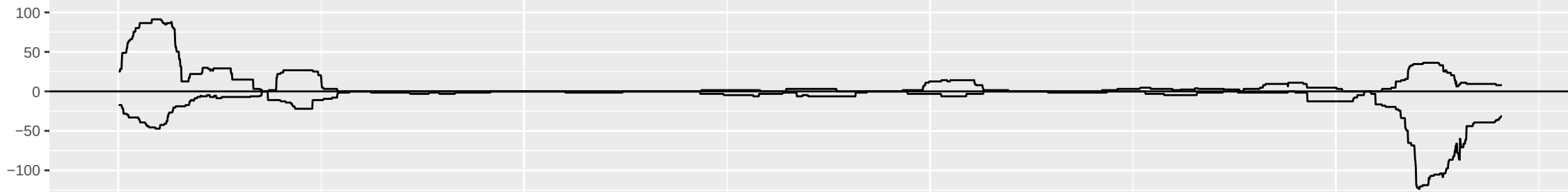
HsBam_piwiKD_68h_B
