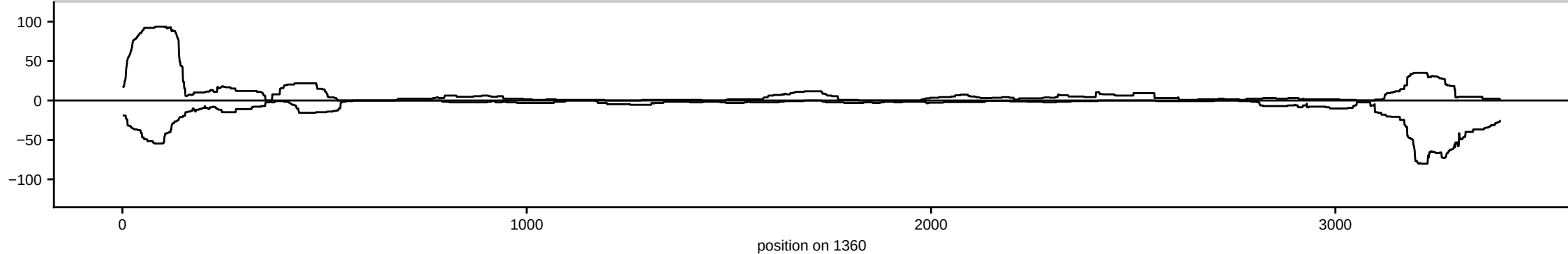
HsBam_polyA_piwiKD_42h_B
