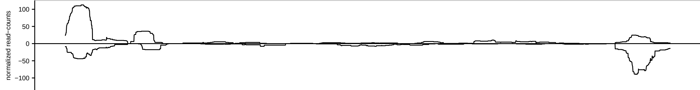
HsBam_polyA_piwiKD_42h_B
