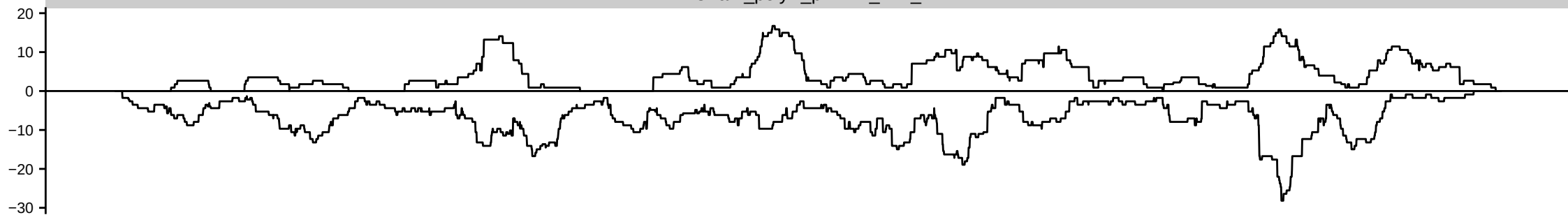
HsBam_polyA_piwiKD_42h_B
