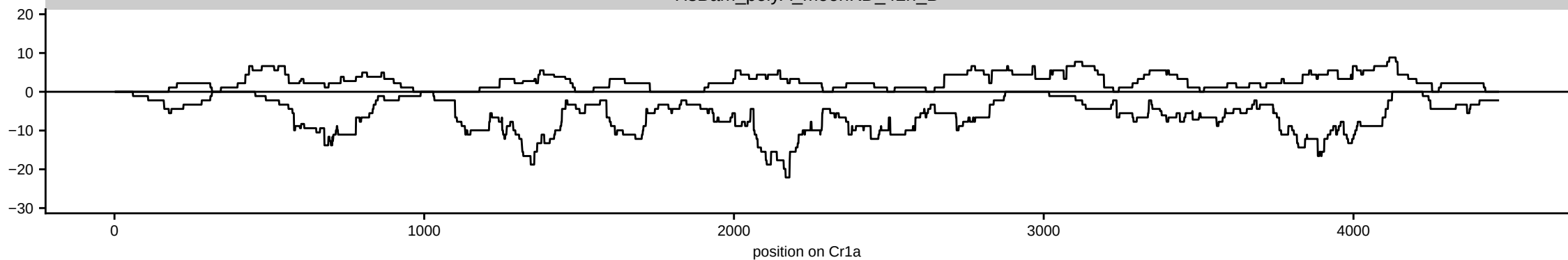
HsBam_polyA_moonKD_42h_B
