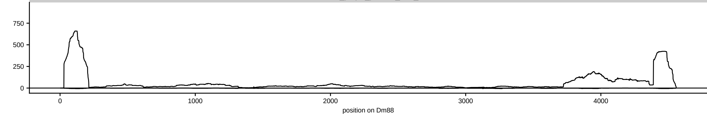
HsBam_polyA_piwiKD_00h_A
