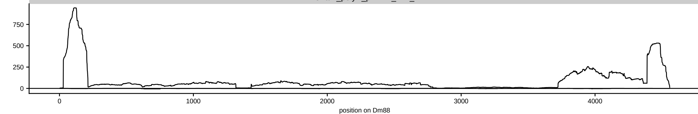
HsBam_polyA_piwiKD_42h_B
