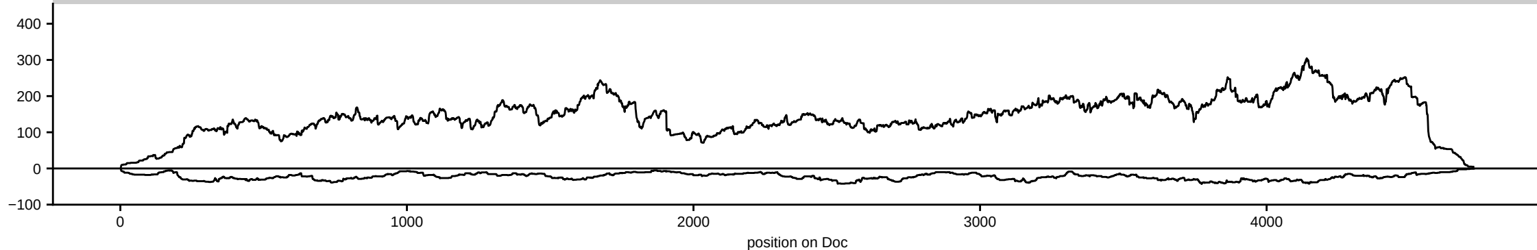
HsBam_polyA_piwiKD_42h_B
