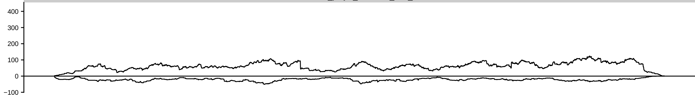
HsBam_polyA_piwiKD_00h_A
