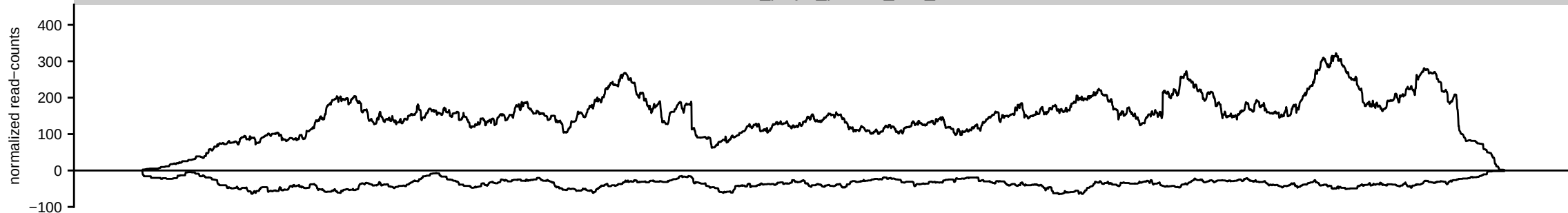
HsBam_polyA_piwiKD_42h_B
