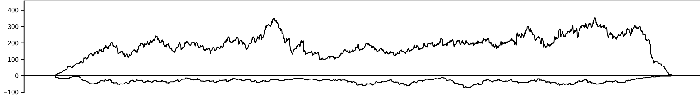
HsBam_polyA_piwiKD_42h_A
