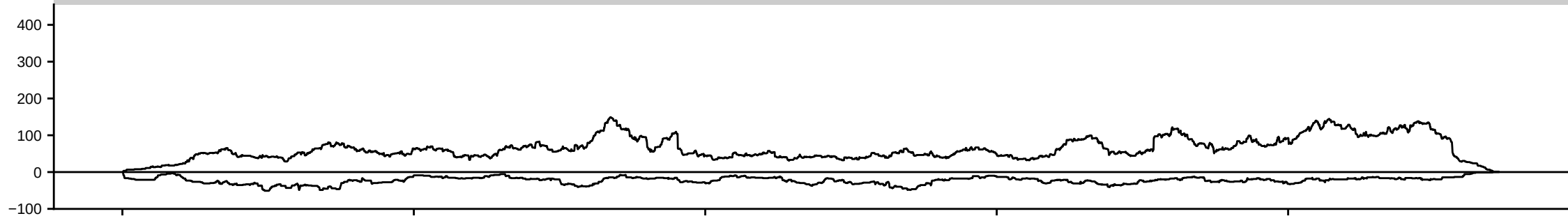
HsBam_polyA_moonKD_42h_B
