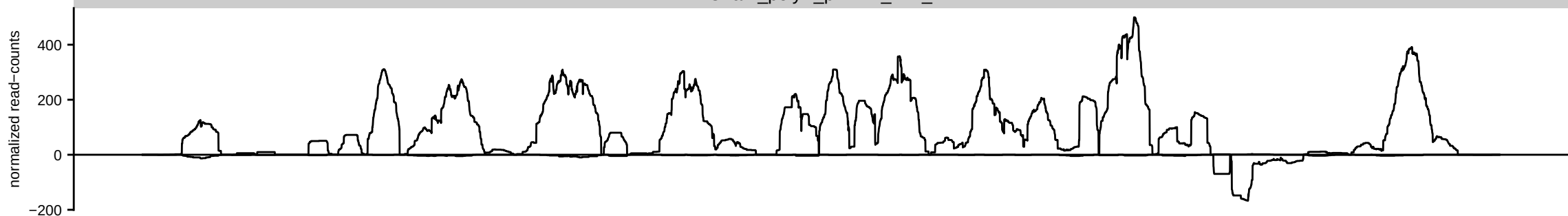
HsBam_polyA_piwiKD_42h_B
