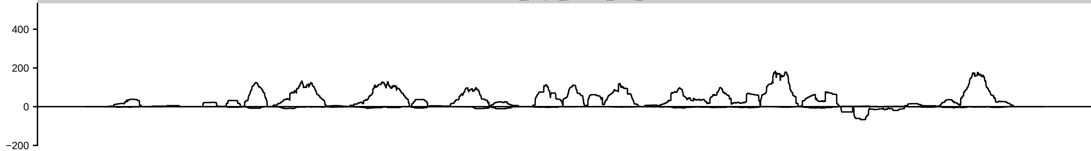
HsBam_polyA_piwiKD_42h_A
