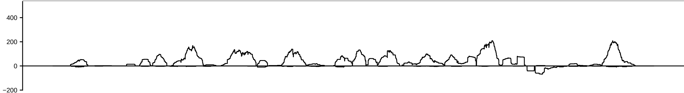
HsBam_piwiKD_68h_B
