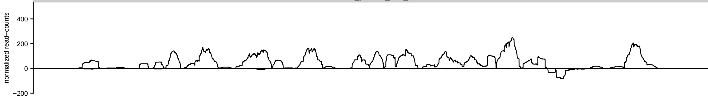
HsBam_polyA_moonKD_00h_A
