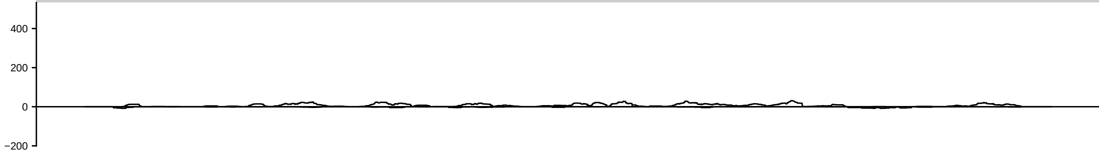
HsBam_polyA_moonKD_68h_B
