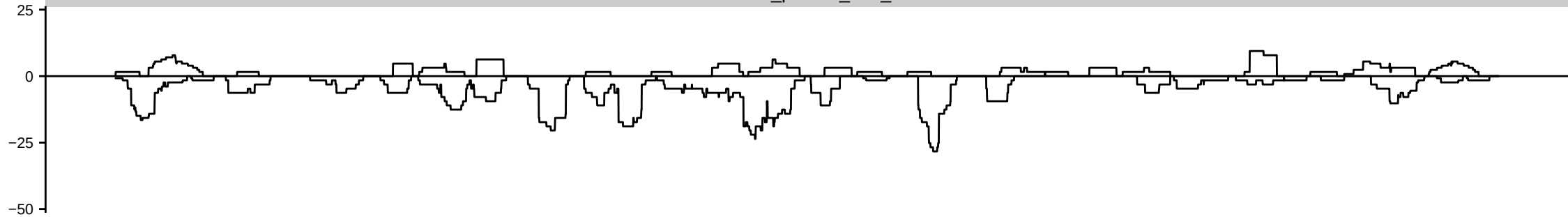
HsBam_piwiKD_68h_B
