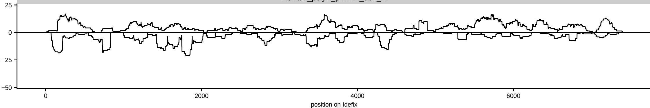
HsBam_polyA_piwiKD_00h_A
