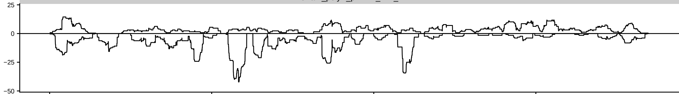
HsBam_polyA_piwiKD_42h_B
