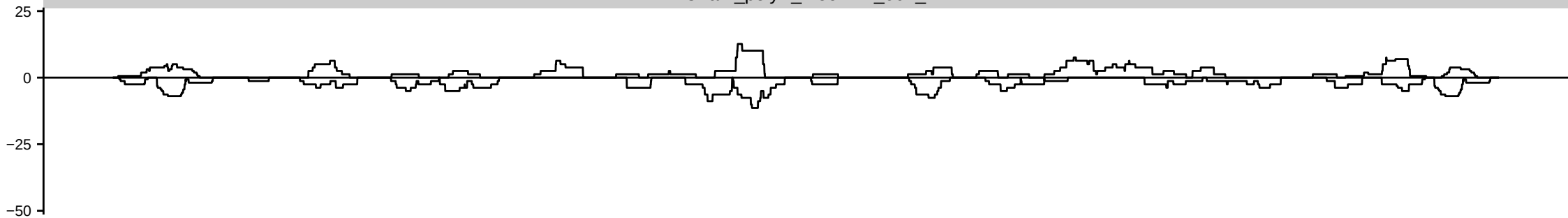
HsBam_polyA_moonKD_42h_A
