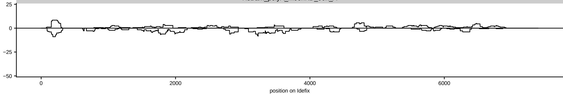
HsBam_polyA_moonKD_00h_A
