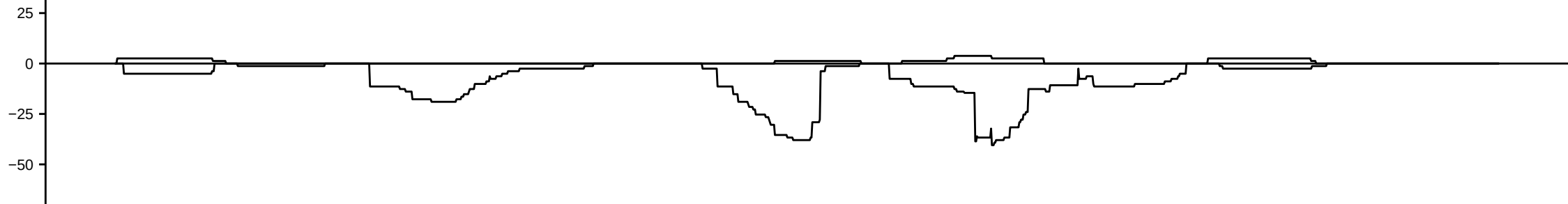
HsBam_polyA_moonKD_42h_A
