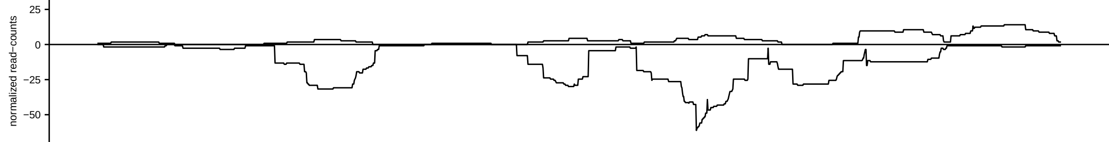
HsBam_polyA_piwiKD_42h_B
