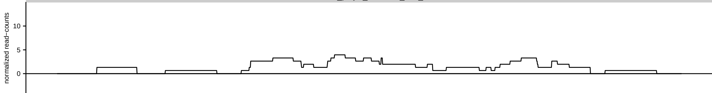
HsBam_polyA_moonKD_42h_B
