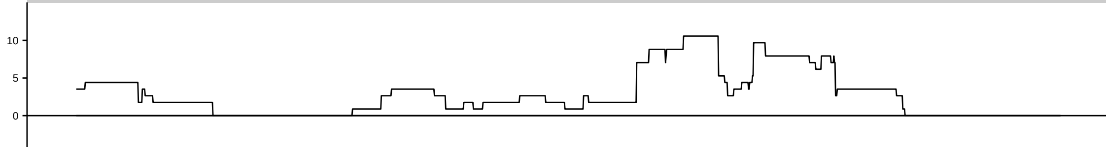
HsBam_polyA_piwiKD_42h_A
