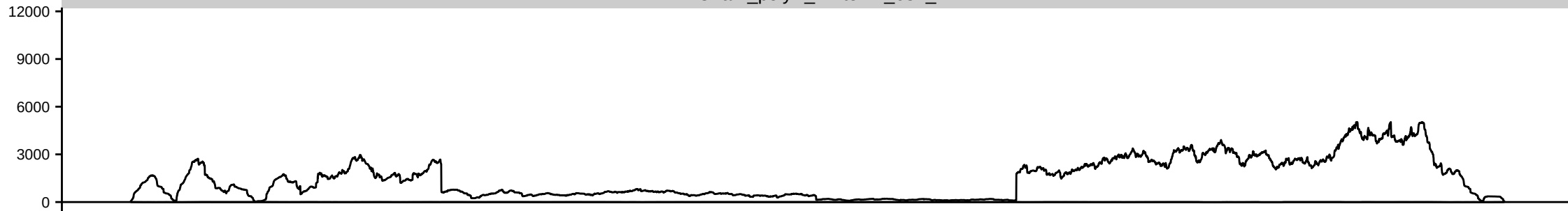
Ov_polyA_piwiKD_A
