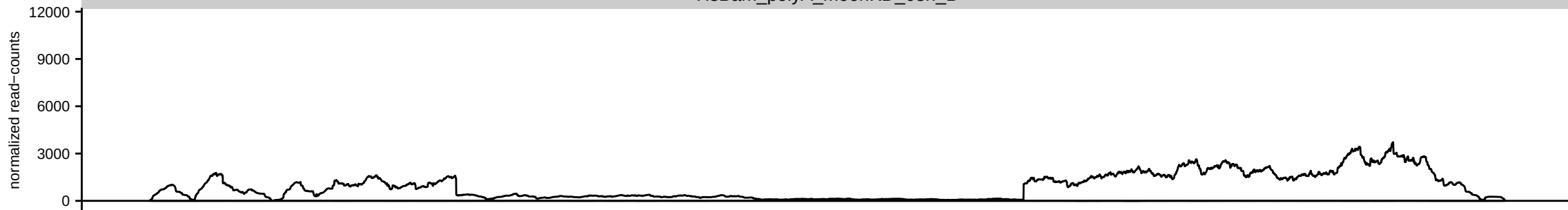
HsBam_polyA_piwiKD_00h_A
