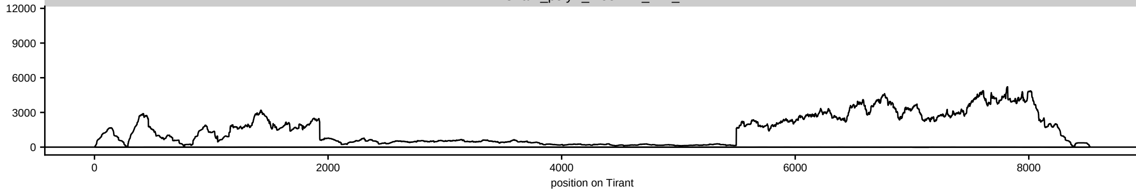
HsBam_polyA_moonKD_42h_B
