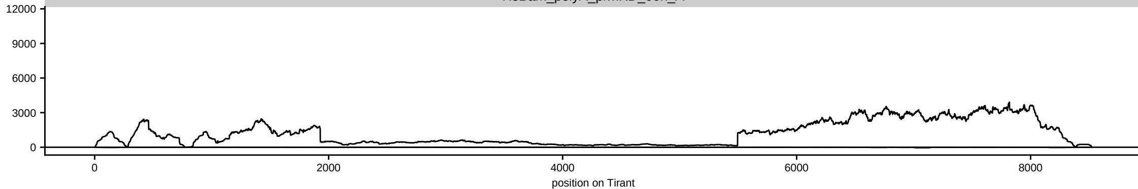
HsBam_polyA_piwiKD_00h_A
