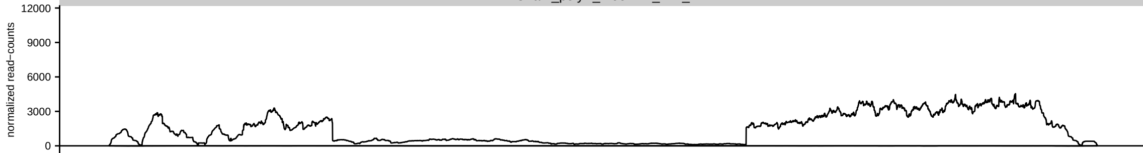
HsBam_polyA_moonKD_42h_B
