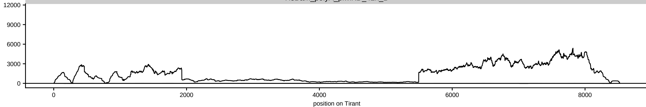
HsBam_polyA_piwiKD_42h_B
