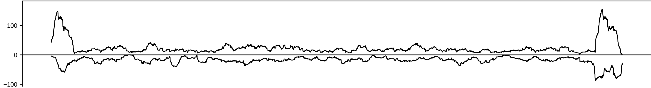
HsBam_polyA_piwiKD_42h_A
