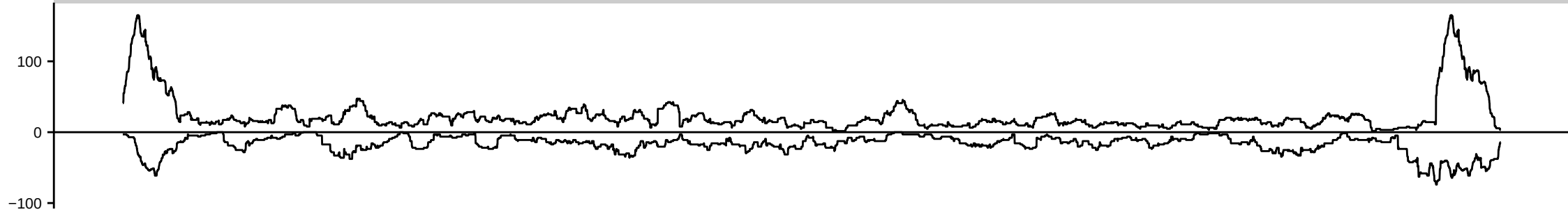
HsBam_piwiKD_68h_B
