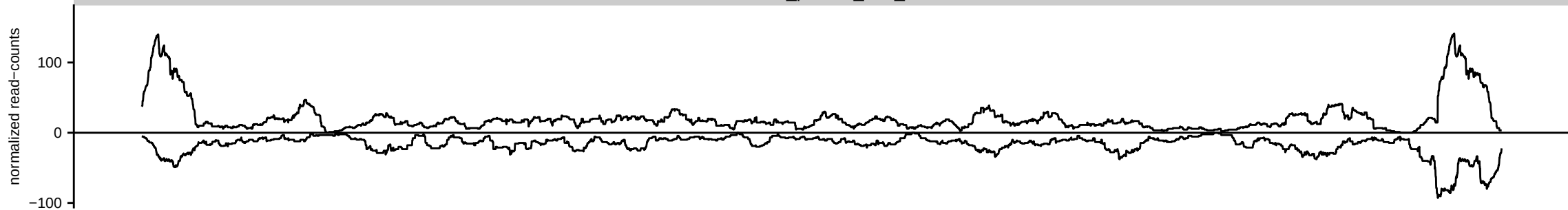
HsBam_polyA_moonKD_00h_A
