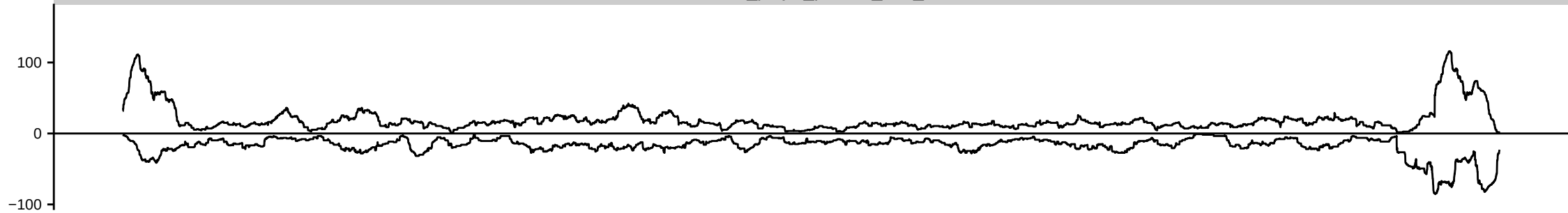
HsBam_polyA_piwiKD_42h_B
