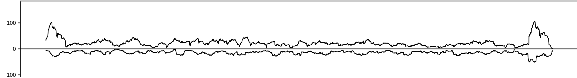
HsBam_polyA_moonKD_42h_B
