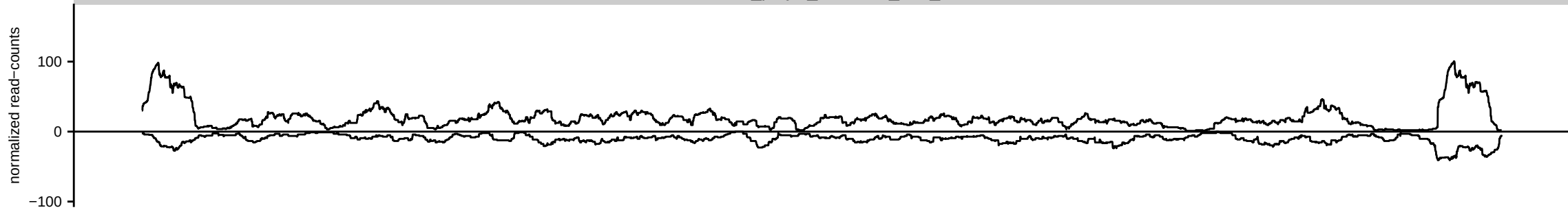
HsBam_polyA_piwiKD_00h_A
