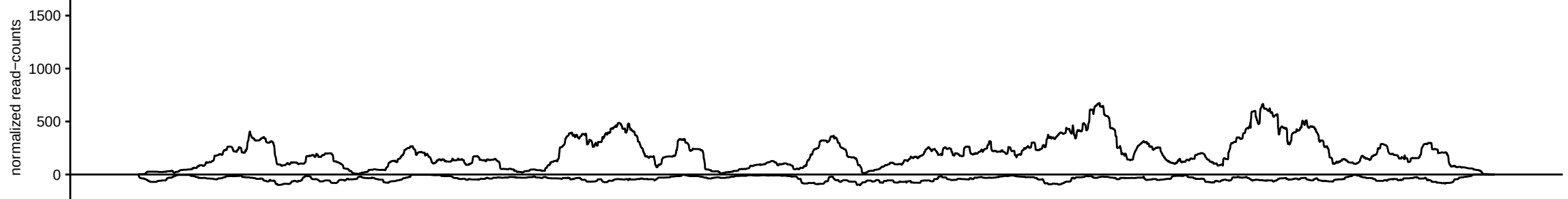
TosK_white_A
