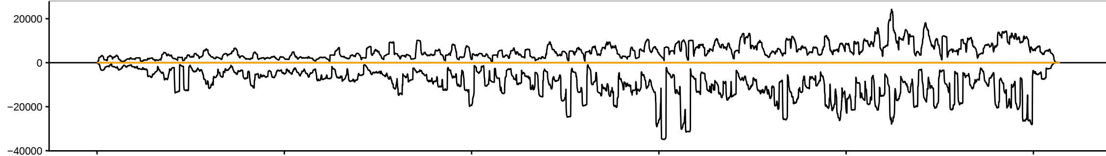
sRNAseq_HsBam_nos_ControlKD_68hAHS_repD_283082_sRBC_TGACT
