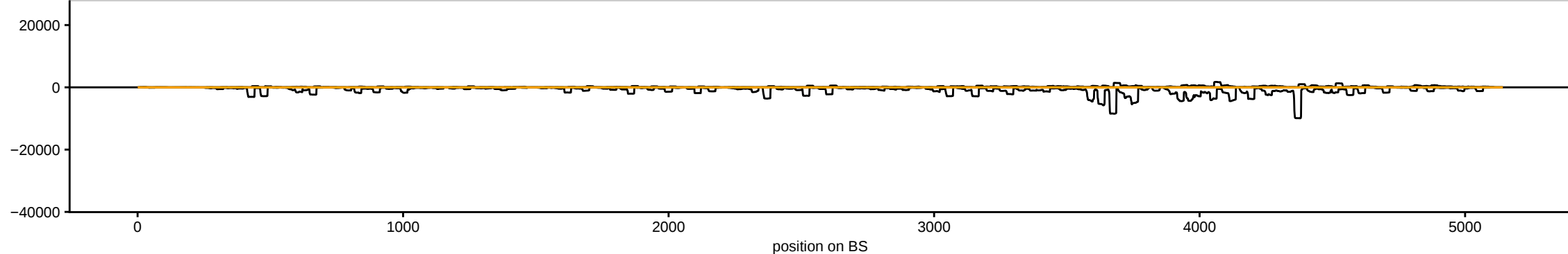
sRNAseq_Ovaries_MTD_PiwiKD_ov_repE_283083_sRBC_ACGAG
