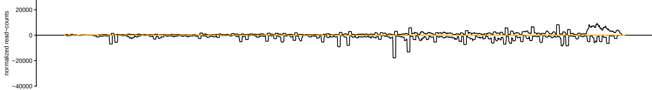
sRNAseq_HsBam_nos_PiwiKD_00hAHS_repD_283082_sRBC_CGTTC
