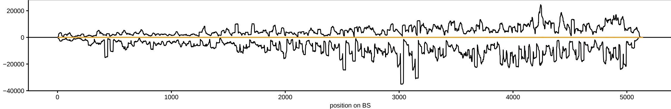
sRNAseq_HsBam_nos_ControlKD_00hAHS_repD_283082_sRBC_GTCAG
