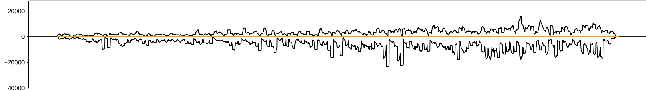
sRNAseq_HsBam_nos_ControlKD_68hAHS_repC_283081_sRBC_AGCAA
