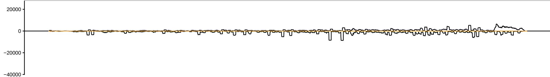
sRNAseq_HsBam_nos_PiwiKD_00hAHS_repC_283081_sRBC_GGTAT
