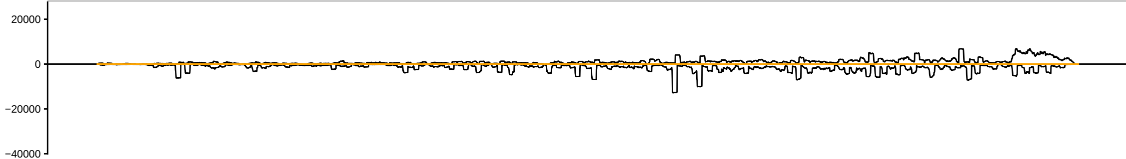
sRNAseq_HsBam_nos_PiwiKD_68hAHS_repC_283081_sRBC_TACCA
