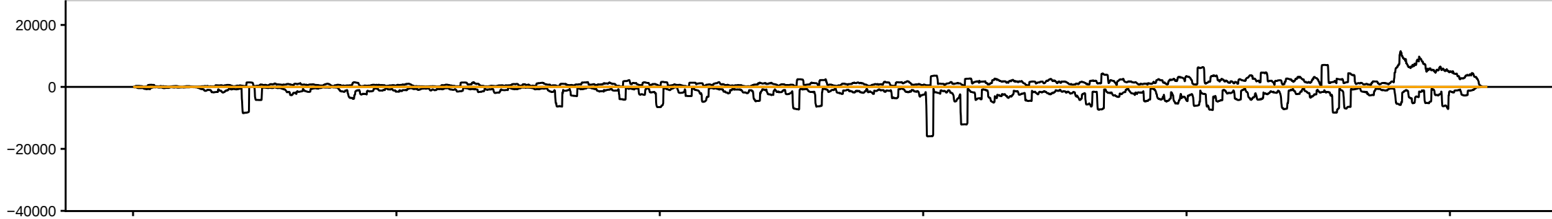
sRNAseq_HsBam_nos_PiwiKD_68hAHS_repD_283082_sRBC_ATGGA
