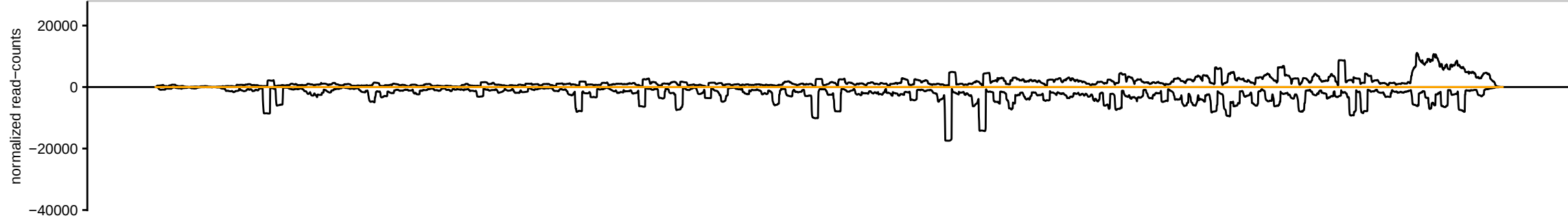
sRNAseq_HsBam_nos_PiwiKD_68hAHS_repD_283082_sRBC_ATGGA
