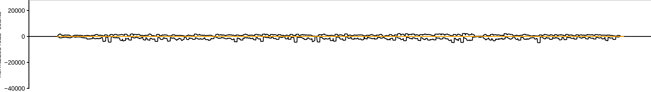
sRNAseq_Ovaries_MTD_PiwiKD_ov_repE_283083_sRBC_ACGAG
