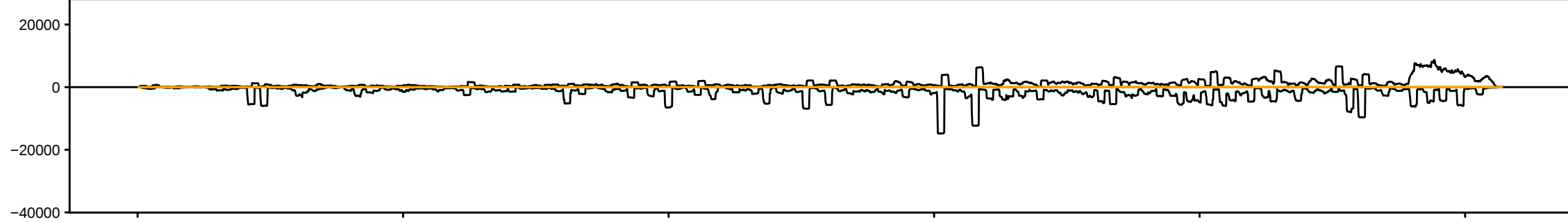
sRNAseq_HsBam_nos_PiwiKD_00hAHS_repD_283082_sRBC_CGTTC
