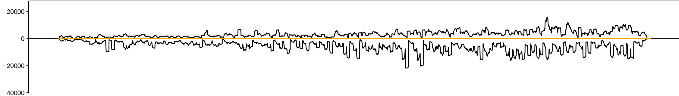
sRNAseq_HsBam_nos_ControlKD_00hAHS_repC_283081_sRBC_CAGTG
