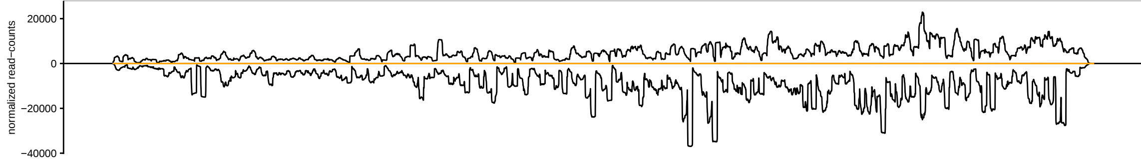
sRNAseq_HsBam_nos_ControlKD_68hAHS_repD_283082_sRBC_TGACT
