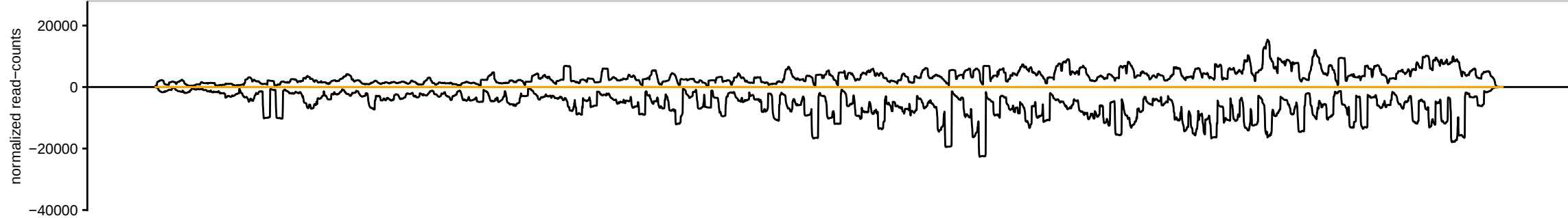
sRNAseq_HsBam_nos_ControlKD_00hAHS_repD_283082_sRBC_GTCAG
