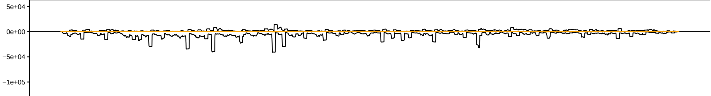
sRNAseq_HsBam_nos_PiwiKD_00hAHS_repC_283081_sRBC_GGTAT
