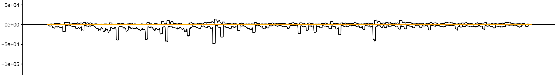
sRNAseq_HsBam_nos_PiwiKD_68hAHS_repC_283081_sRBC_TACCA
