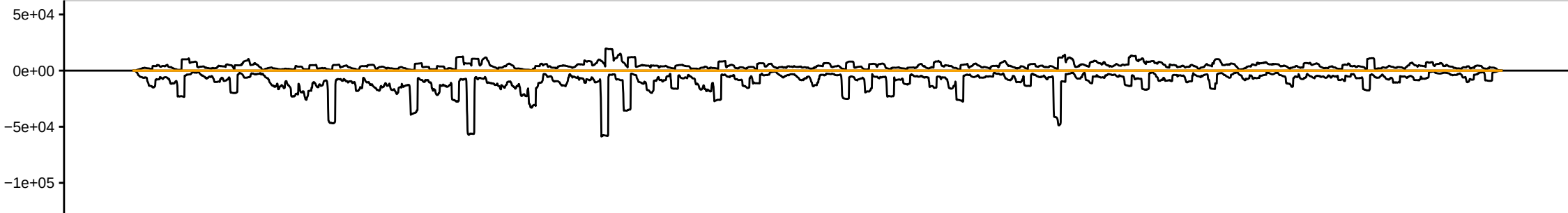
sRNAseq_HsBam_nos_PiwiKD_68hAHS_repD_283082_sRBC_ATGGA
