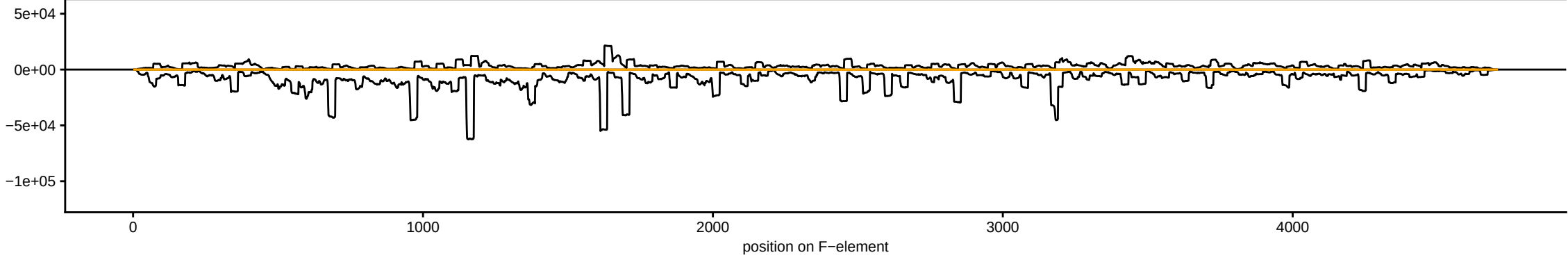
sRNAseq_HsBam_nos_PiwiKD_00hAHS_repD_283082_sRBC_CGTTC
