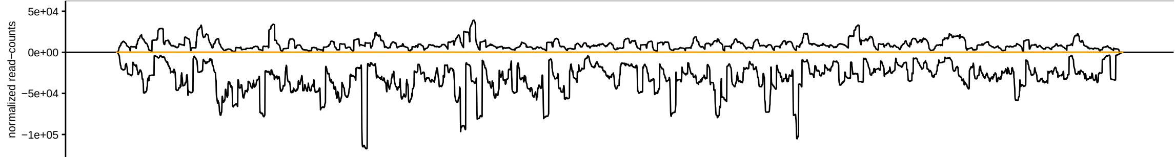
sRNAseq_HsBam_nos_ControlKD_68hAHS_repD_283082_sRBC_TGACT
