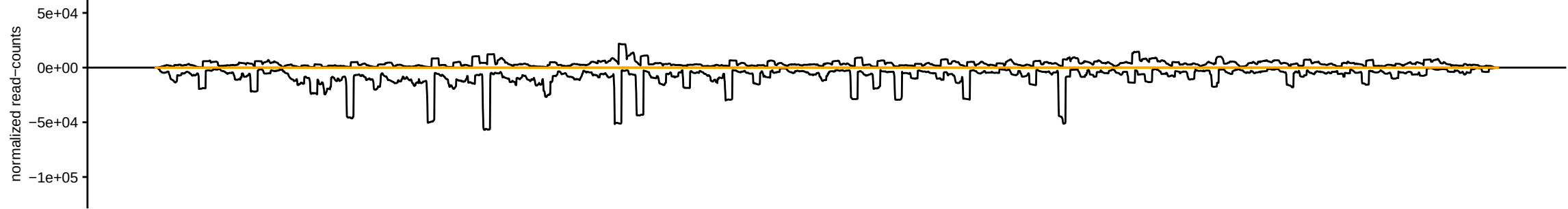
sRNAseq_HsBam_nos_PiwiKD_00hAHS_repD_283082_sRBC_CGTTC
