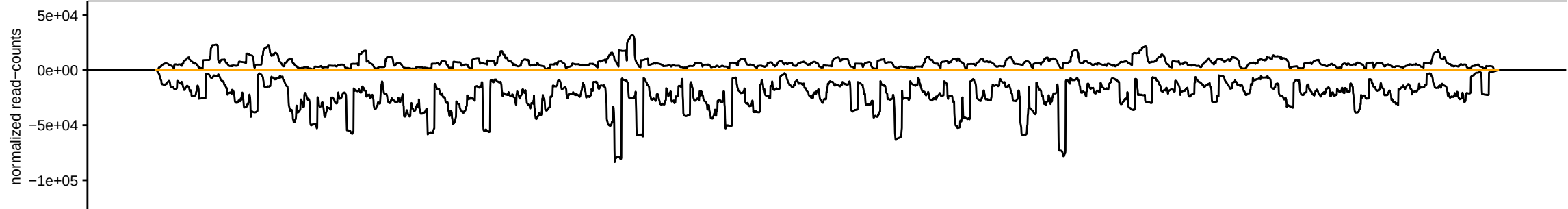
sRNAseq_HsBam_nos_ControlKD_00hAHS_repD_283082_sRBC_GTCAG
