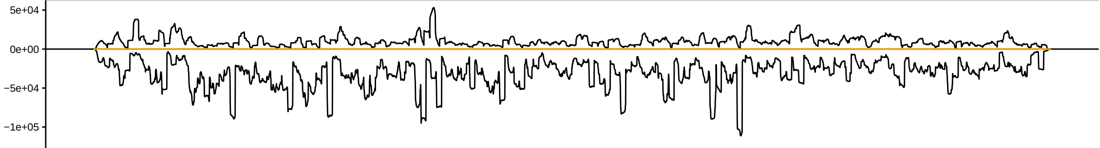
sRNAseq_HsBam_nos_ControlKD_00hAHS_repD_283082_sRBC_GTCAG
