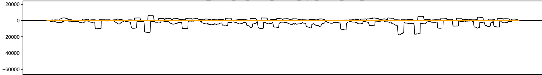
sRNAseq_HsBam_nos_PiwiKD_00hAHS_repD_283082_sRBC_CGTTC
