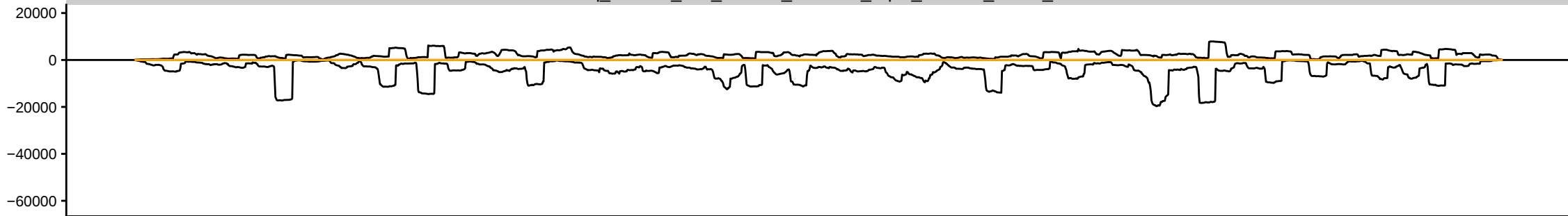
sRNAseq_HsBam_nos_PiwiKD_68hAHS_repD_283082_sRBC_ATGGA
