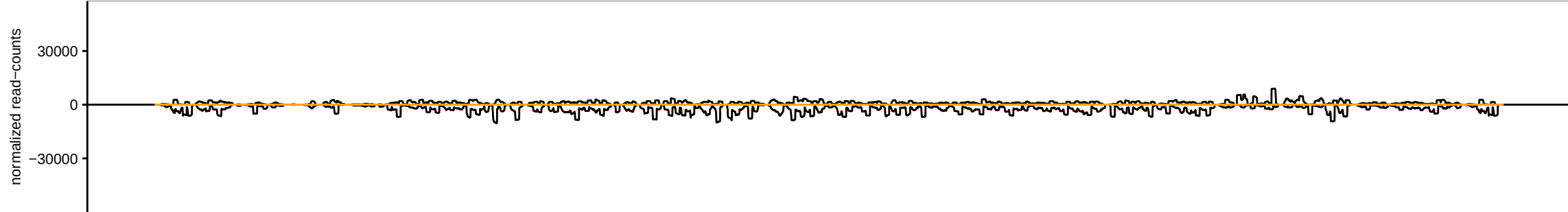
sRNAseq_Ovaries_MTD_PiwiKD_ov_repE_283083_sRBC_ACGAG
