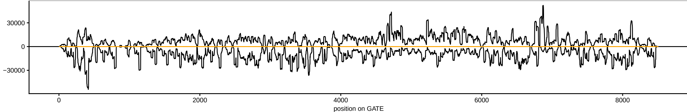
sRNAseq_HsBam_nos_ControlKD_68hAHS_repD_283082_sRBC_TGACT
