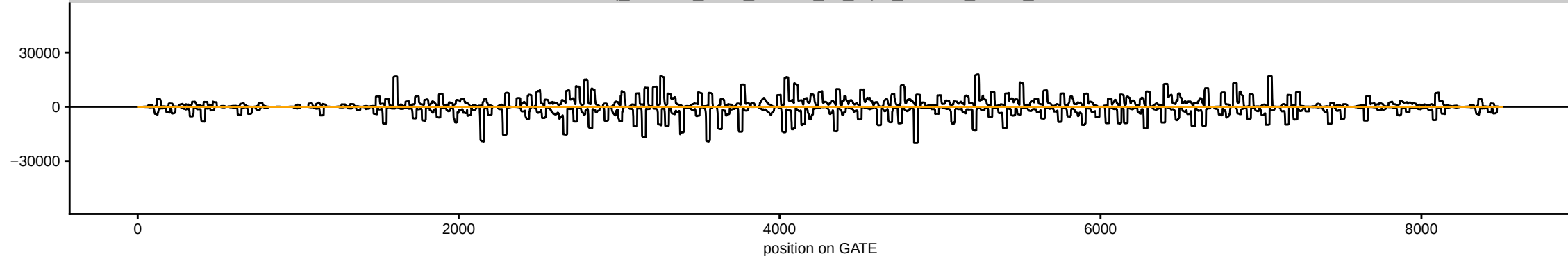
sRNAseq_Ovaries_MTD_PiwiKD_ov_repE_283083_sRBC_ACGAG
