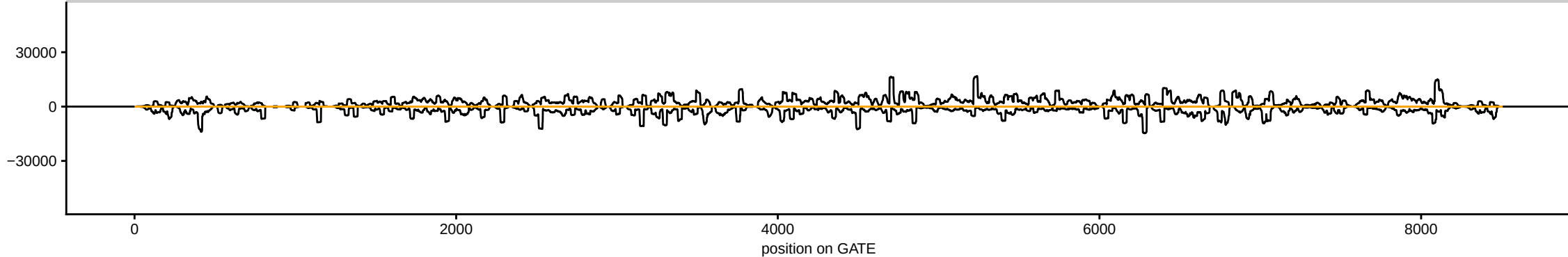
sRNAseq_HsBam_nos_PiwiKD_68hAHS_repD_283082_sRBC_ATGGA
