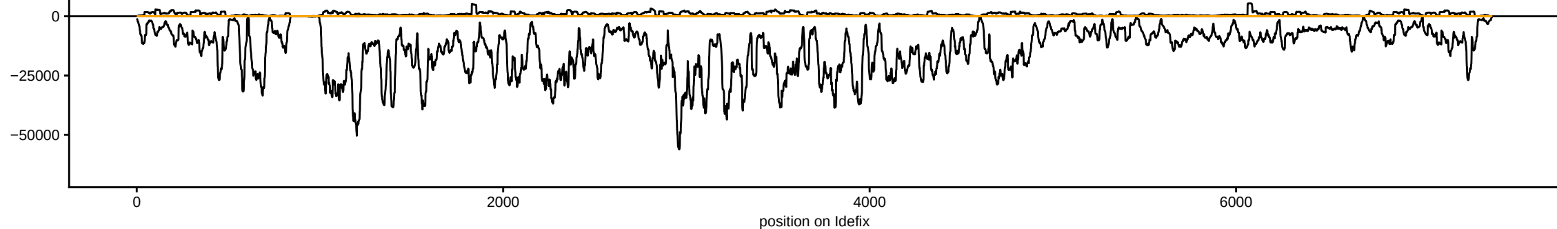
sRNAseq_HsBam_nos_PiwiKD_68hAHS_repD_283082_sRBC_ATGGA
