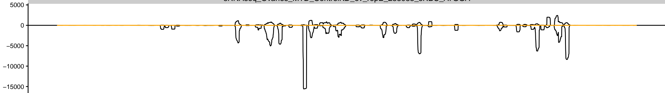
sRNAseq_Ovaries_MTD_ControlKD_ov_repF_283083_sRBC_GAACG
