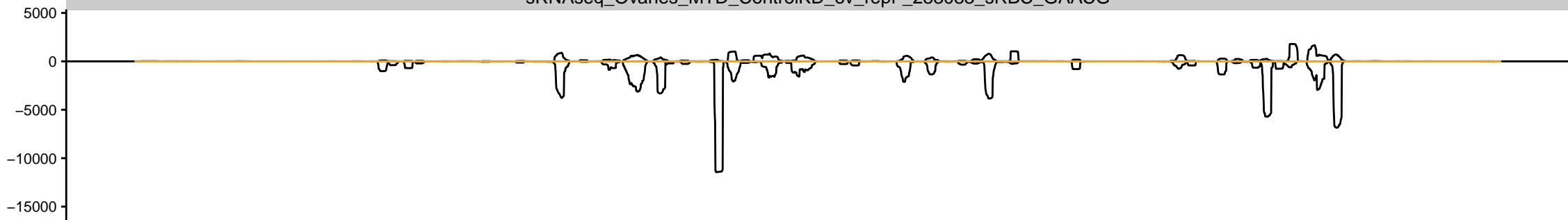
sRNAseq_Ovaries_MTD_PiwiKD_ov_repE_283083_sRBC_ACGAG
