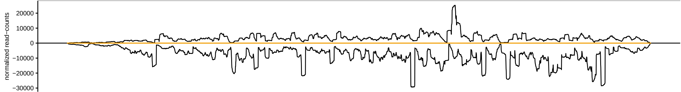
sRNAseq_HsBam_nos_ControlKD_68hAHS_repD_283082_sRBC_TGACT
