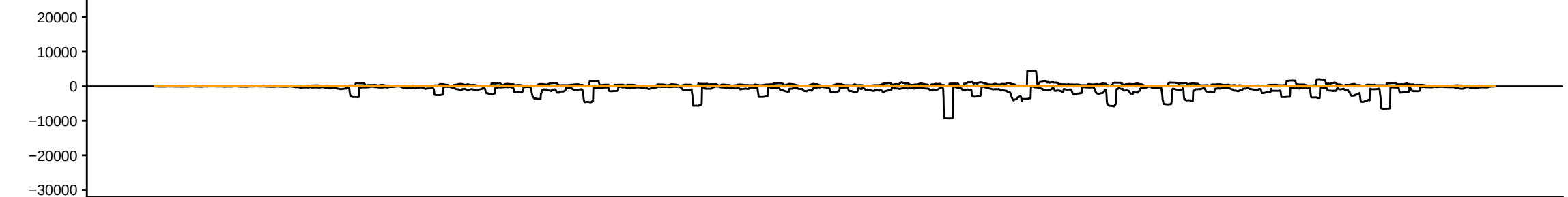
sRNAseq_HsBam_nos_PiwiKD_00hAHS_repD_283082_sRBC_CGTTC
