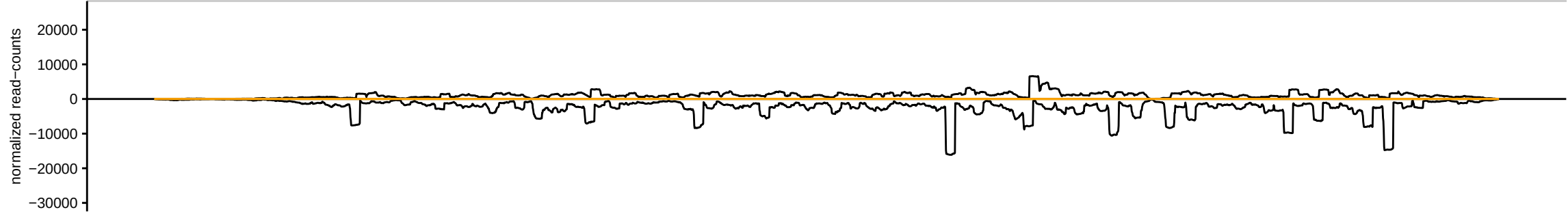
sRNAseq_HsBam_nos_PiwiKD_68hAHS_repD_283082_sRBC_ATGGA
