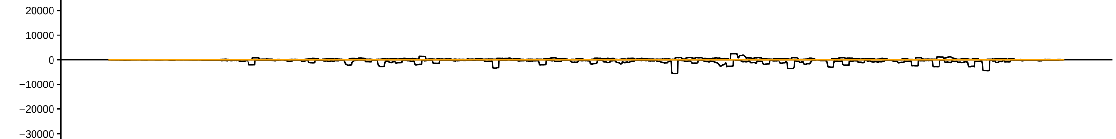
sRNAseq_HsBam_nos_PiwiKD_00hAHS_repC_283081_sRBC_GGTAT
