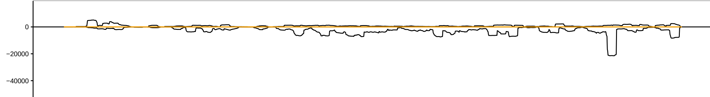
sRNAseq_Ovaries_MTD_ControlKD_ov_repF_283083_sRBC_GAACG
