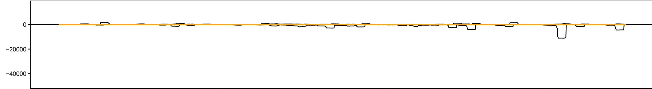
sRNAseq_Ovaries_MTD_PiwiKD_ov_repE_283083_sRBC_ACGAG
