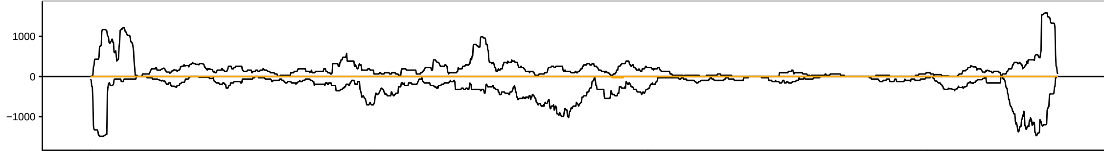
sRNAseq_HsBam_nos_ControlKD_00hAHS_repD_283082_sRBC_GTCAG
