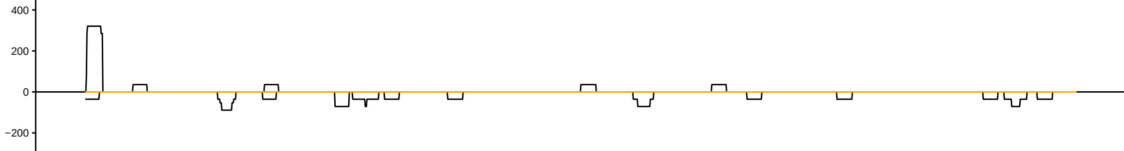
sRNAseq_HsBam_nos_PiwiKD_68hAHS_repD_283082_sRBC_ATGGA
