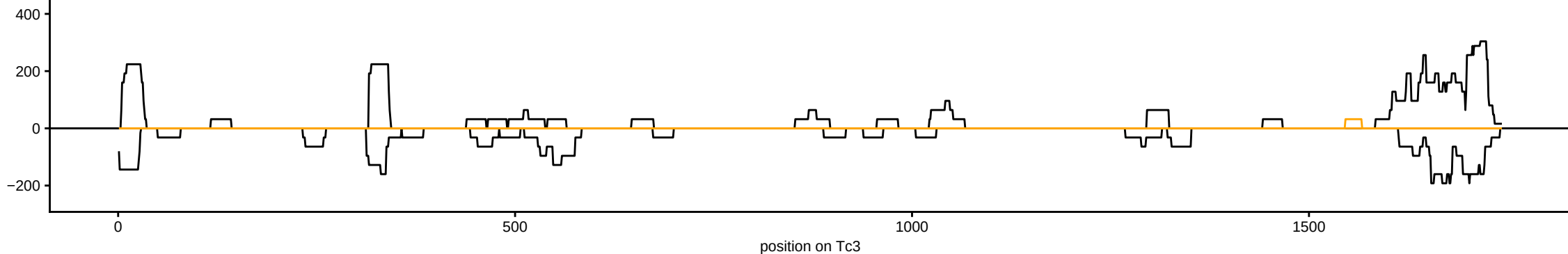
sRNAseq_HsBam_nos_ControlKD_00hAHS_repD_283082_sRBC_GTCAG
