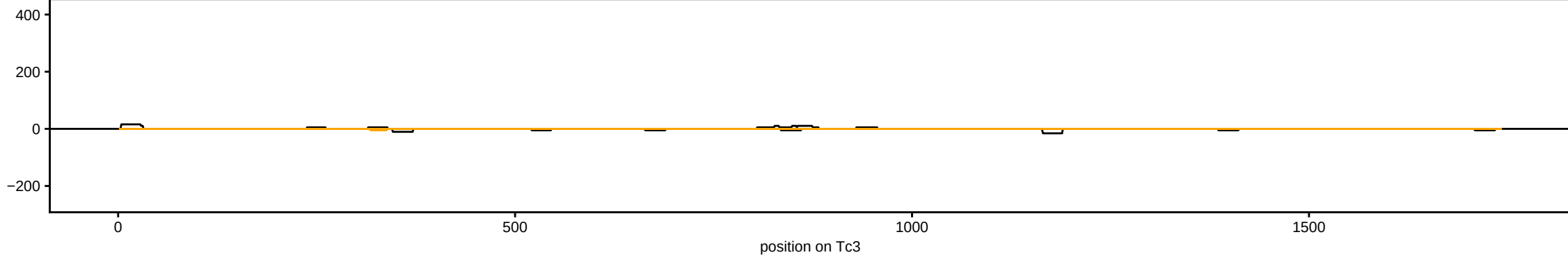
sRNAseq_Ovaries_MTD_PiwiKD_ov_repE_283083_sRBC_ACGAG
