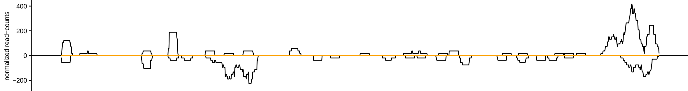
sRNAseq_HsBam_nos_ControlKD_68hAHS_repD_283082_sRBC_TGACT
