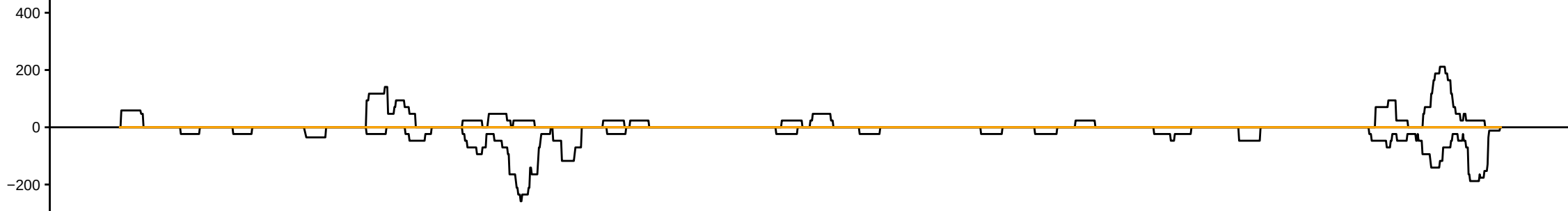
sRNAseq_HsBam_nos_ControlKD_00hAHS_repC_283081_sRBC_CAGTG
