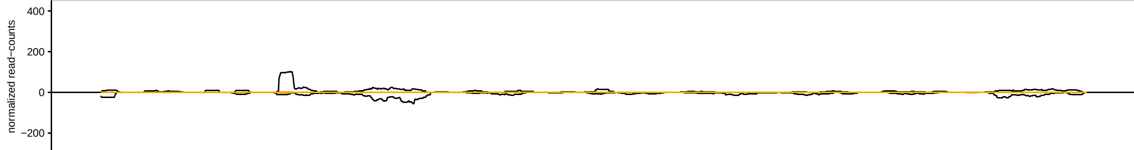
sRNAseq_Ovaries_MTD_PiwiKD_ov_repE_283083_sRBC_ACGAG
