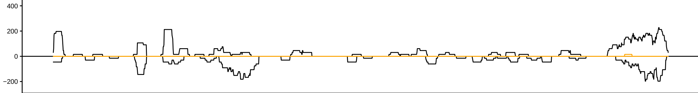
sRNAseq_HsBam_nos_ControlKD_68hAHS_repD_283082_sRBC_TGACT
