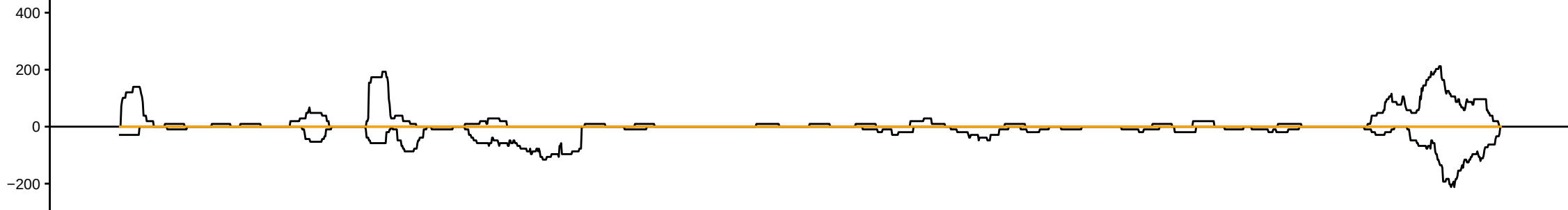
sRNAseq_HsBam_nos_ControlKD_68hAHS_repC_283081_sRBC_AGCAA
