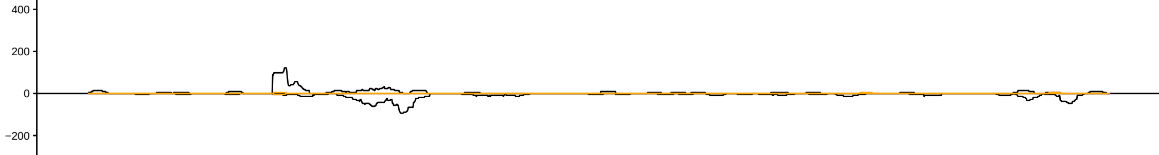
sRNAseq_Ovaries_MTD_ControlKD_ov_repF_283083_sRBC_GAACG
