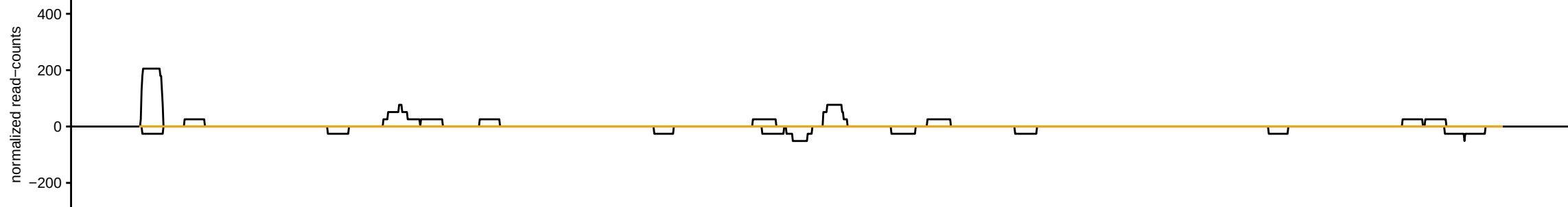
sRNAseq_HsBam_nos_PiwiKD_68hAHS_repD_283082_sRBC_ATGGA
