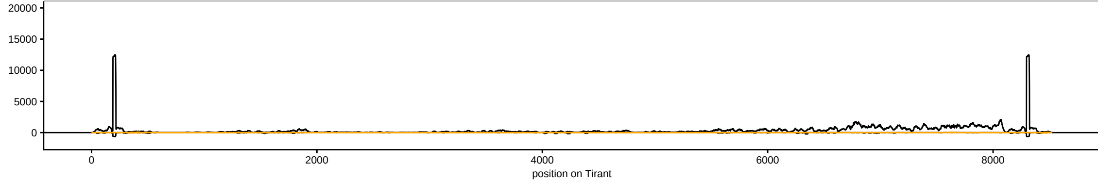
sRNAseq_HsBam_nos_PiwiKD_68hAHS_repD_283082_sRBC_ATGGA
