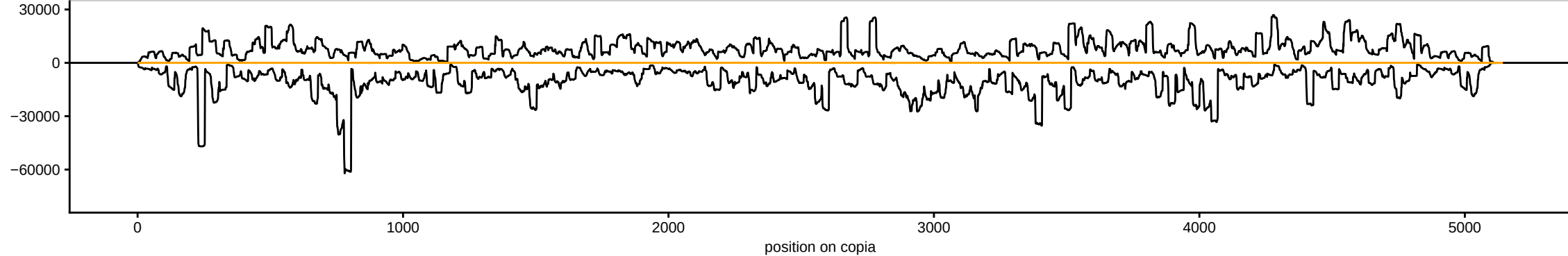
sRNAseq_HsBam_nos_ControlKD_00hAHS_repD_283082_sRBC_GTCAG
