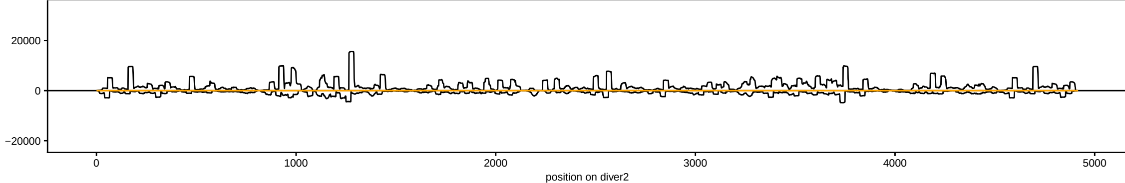
sRNAseq_HsBam_nos_PiwiKD_00hAHS_repD_283082_sRBC_CGTTTC
