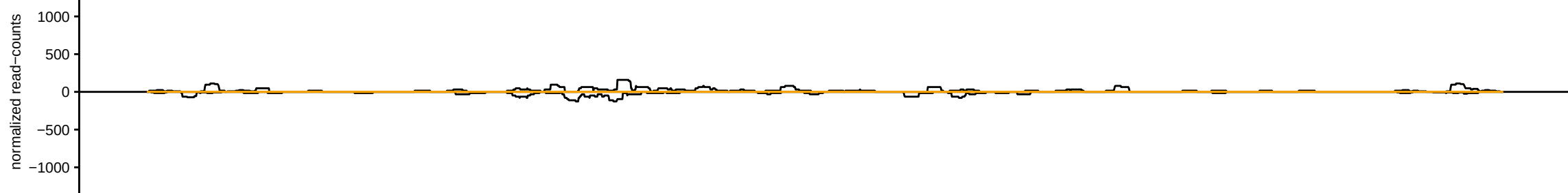
sRNAseq_HsBam_nos_PiwiKD_00hAHS_repD_283082_sRBC_CGTTC
