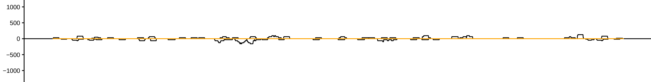
sRNAseq_HsBam_nos_PiwiKD_00hAHS_repD_283082_sRBC_CGTTC
