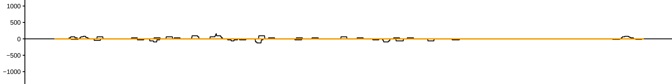
sRNAseq_HsBam_nos_PiwiKD_00hAHS_repC_283081_sRBC_GGTAT
