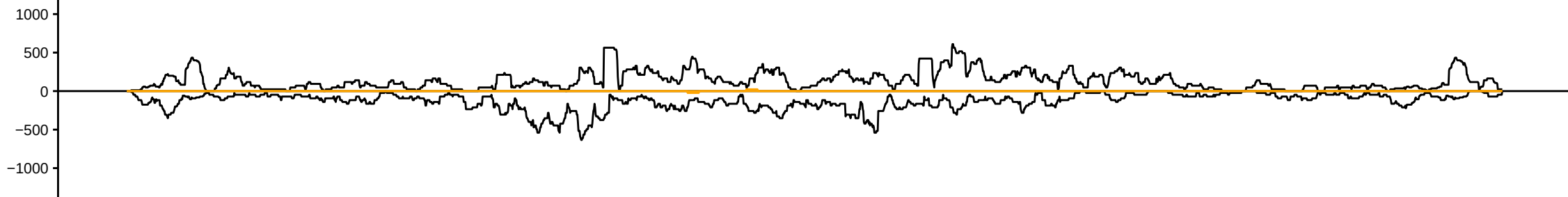
sRNAseq_HsBam_nos_ControlKD_00hAHS_repC_283081_sRBC_CAGTG
