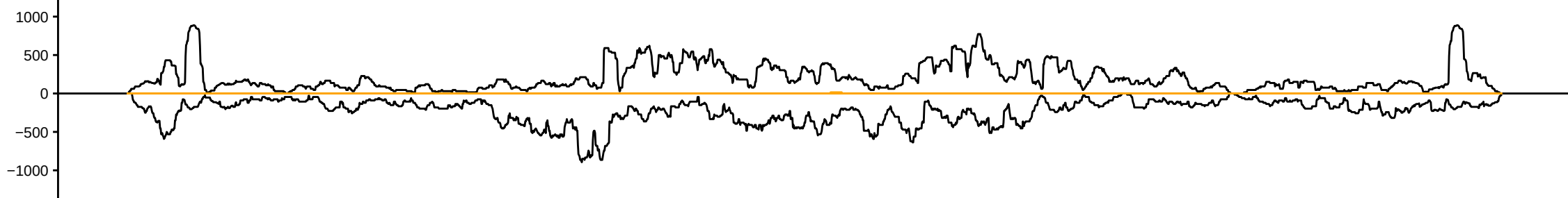
sRNAseq_HsBam_nos_ControlKD_68hAHS_repD_283082_sRBC_TGACT
