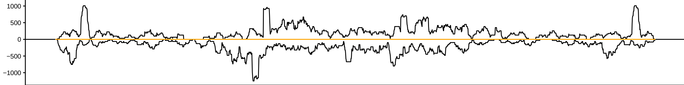
sRNAseq_HsBam_nos_ControlKD_00hAHS_repD_283082_sRBC_GTCAG
