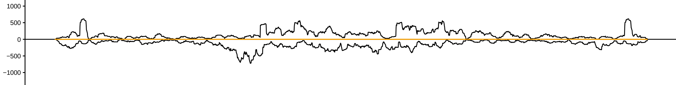
sRNAseq_HsBam_nos_ControlKD_68hAHS_repC_283081_sRBC_AGCAA
