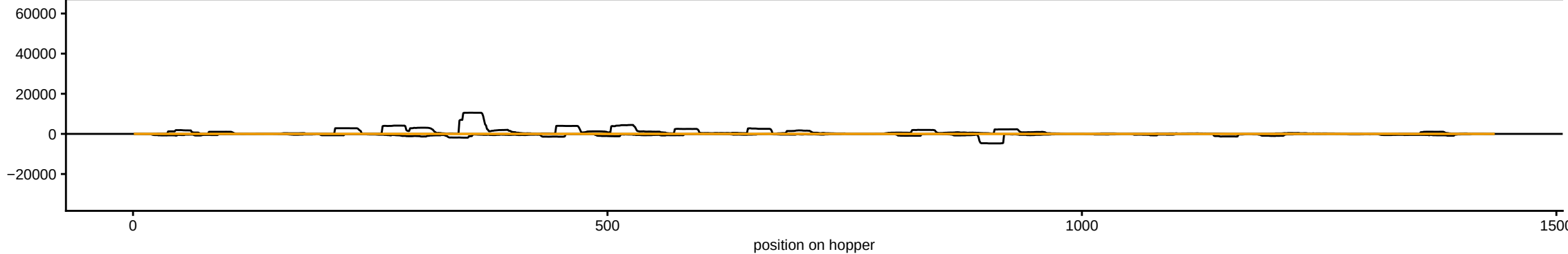
sRNAseq_HsBam_nos_PiwiKD_00hAHS_repD_283082_sRBC_CGTTC
