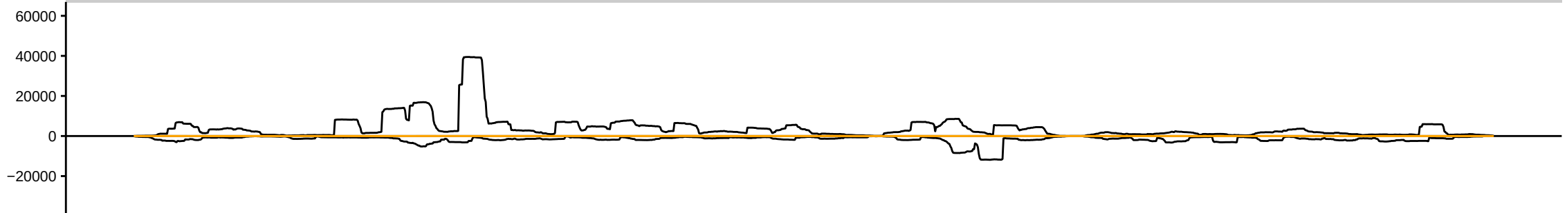
sRNAseq_HsBam_nos_ControlKD_00hAHS_repC_283081_sRBC_CAGTG
