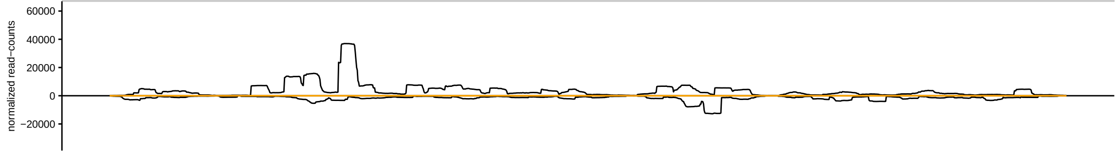
sRNAseq_HsBam_nos_ControlKD_00hAHS_repD_283082_sRBC_GTCAG
