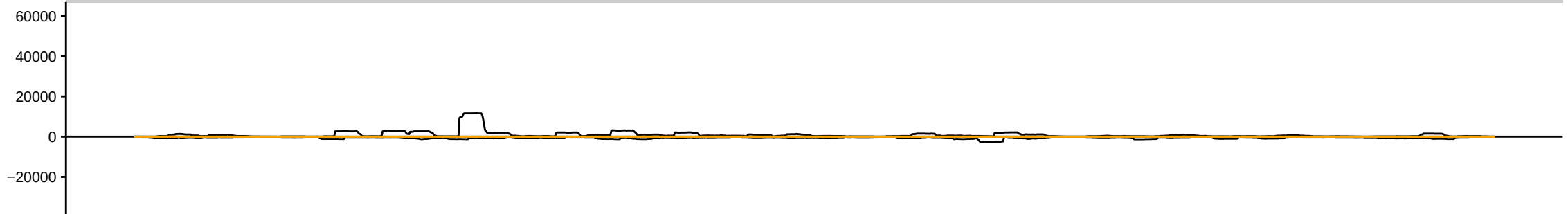
sRNAseq_HsBam_nos_PiwiKD_68hAHS_repC_283081_sRBC_TACCA
