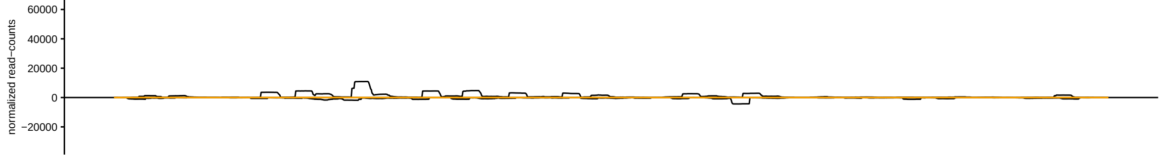
sRNAseq_HsBam_nos_PiwiKD_00hAHS_repD_283082_sRBC_CGTTC
