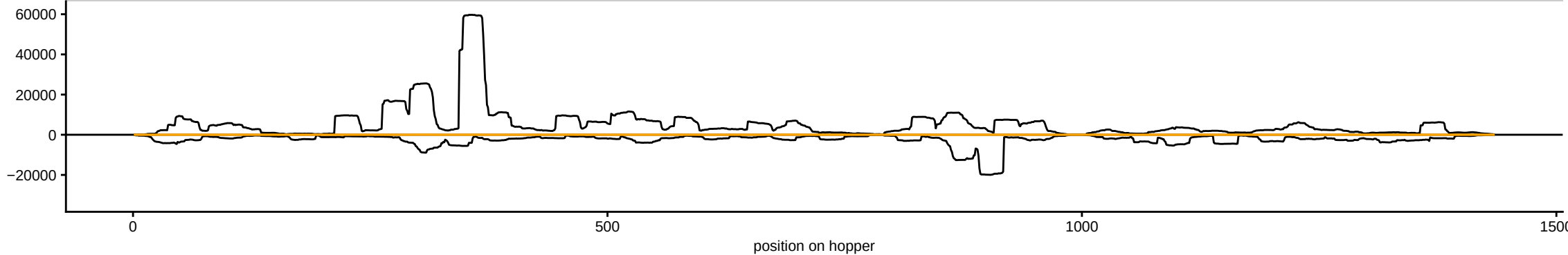
sRNAseq_HsBam_nos_ControlKD_00hAHS_repD_283082_sRBC_GTCAG
