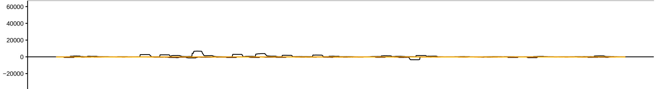
sRNAseq_HsBam_nos_PiwiKD_00hAHS_repC_283081_sRBC_GGTAT
