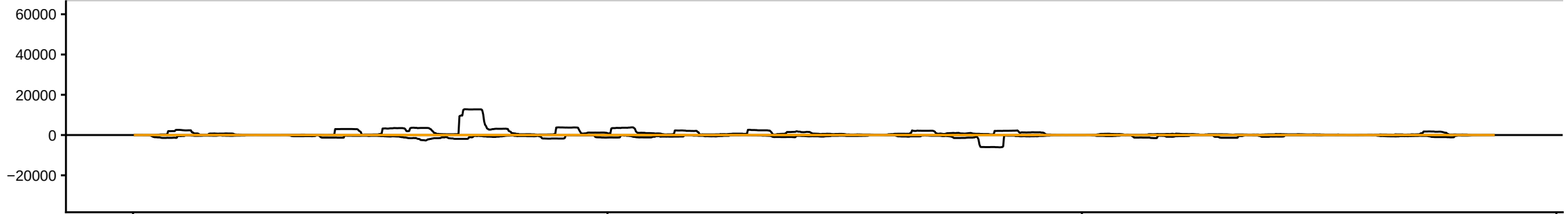
sRNAseq_HsBam_nos_PiwiKD_68hAHS_repD_283082_sRBC_ATGGA
