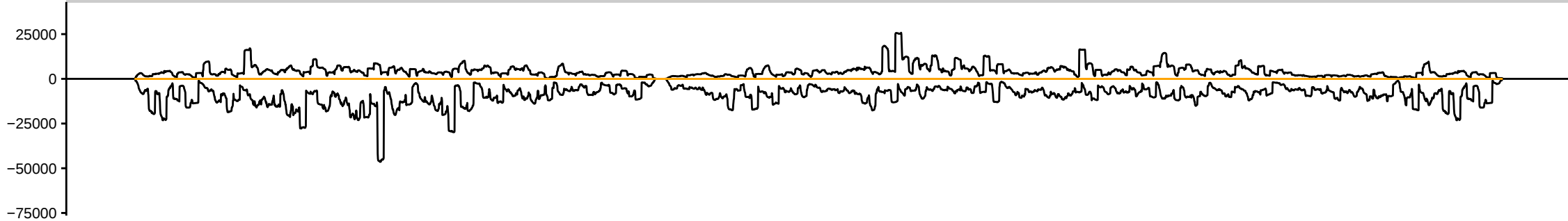
sRNAseq_HsBam_nos_ControlKD_68hAHS_repC_283081_sRBC_AGCAA
