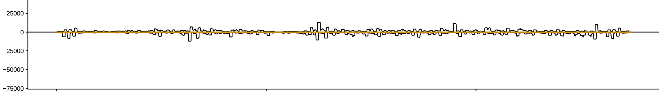
sRNAseq_HsBam_nos_PiwiKD_00hAHS_repD_283082_sRBC_CGTTC
