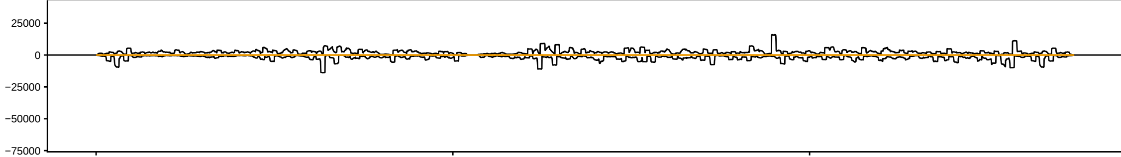
sRNAseq_HsBam_nos_PiwiKD_68hAHS_repD_283082_sRBC_ATGGA
