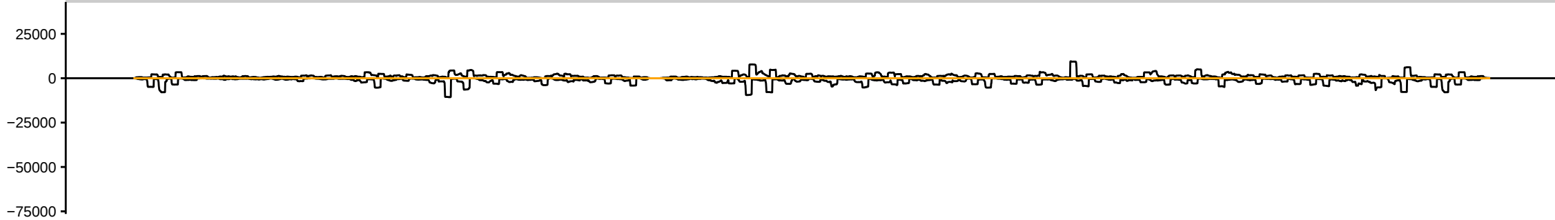
sRNAseq_HsBam_nos_PiwiKD_00hAHS_repC_283081_sRBC_GGTAT
