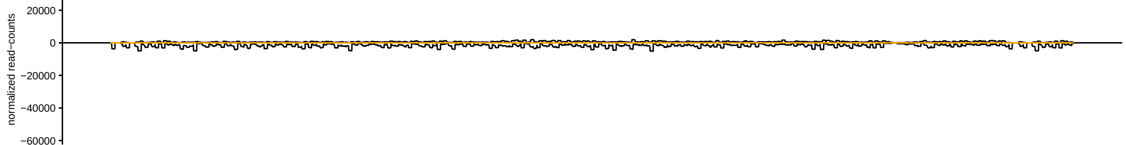
sRNAseq_Ovaries_MTD_PiwiKD_ov_repE_283083_sRBC_ACGAG
