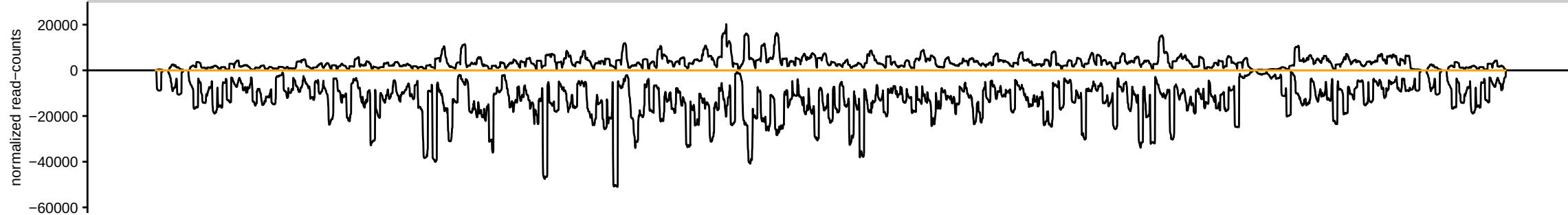
sRNAseq_HsBam_nos_ControlKD_68hAHS_repD_283082_sRBC_TGACT
