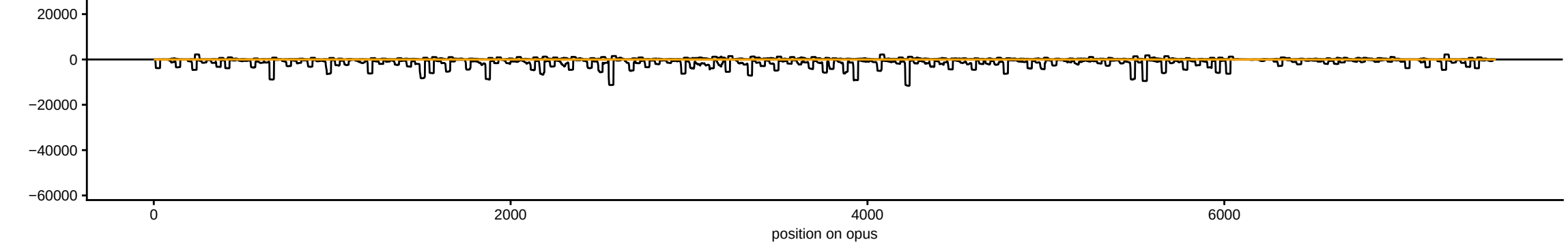
sRNAseq_Ovaries_MTD_PiwiKD_ov_repE_283083_sRBC_ACGAG
