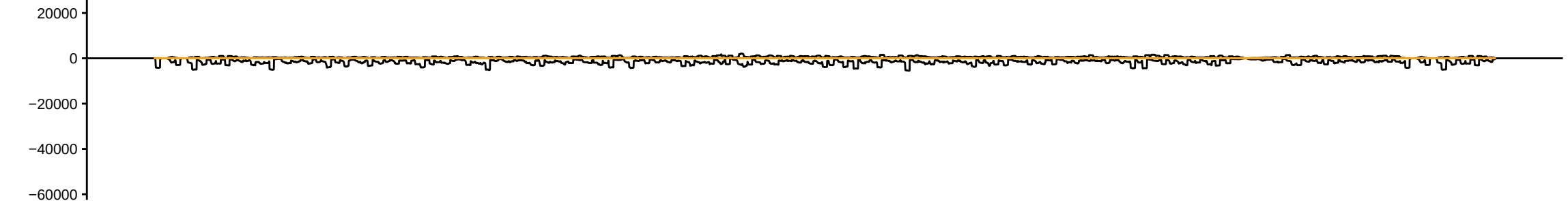
sRNAseq_Ovaries_MTD_ControlKD_ov_repF_283083_sRBC_GAACG
