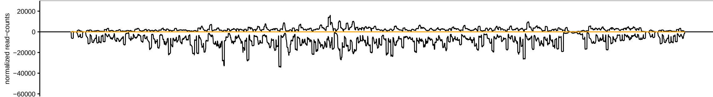
sRNAseq_HsBam_nos_ControlKD_00hAHS_repD_283082_sRBC_GTCAG
