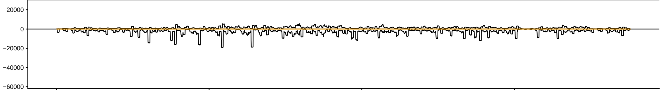
sRNAseq_HsBam_nos_PiwiKD_68hAHS_repD_283082_sRBC_ATGGA
